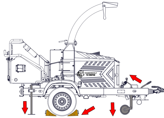
Figure 5 - Chipper in Unhitched Configuration
