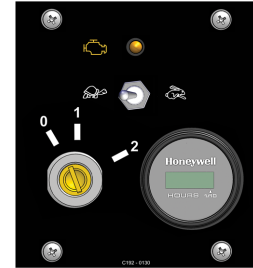
Figure 12 - Control Panel
