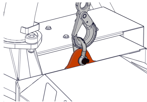
Figure 19 - Lifting Eye and Shackle
