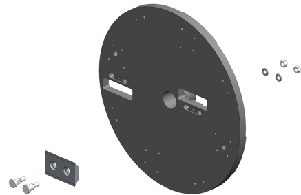
Figure 22 - Blade Mounting
