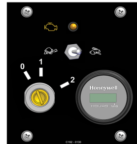
Figure 13 - Throttle Switch
