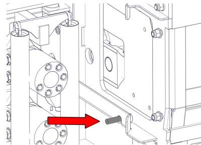
Figure 21 - Locking Bar Inserted
