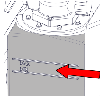
Figure 18 - Hydraulic Oil Level Indicator
