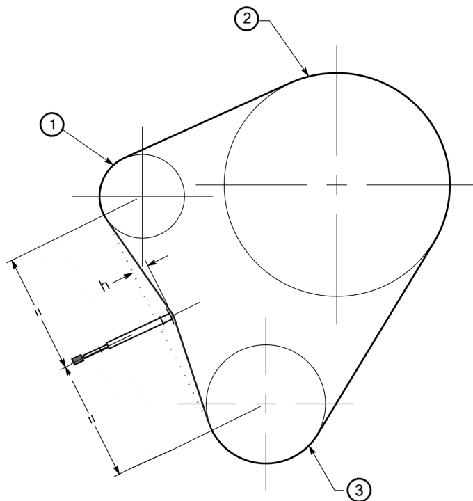
Figure 25 - Rotor Drive Belt Layout
