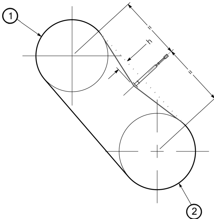
Figure 26 - Hydraulic Pump Belt Layout
